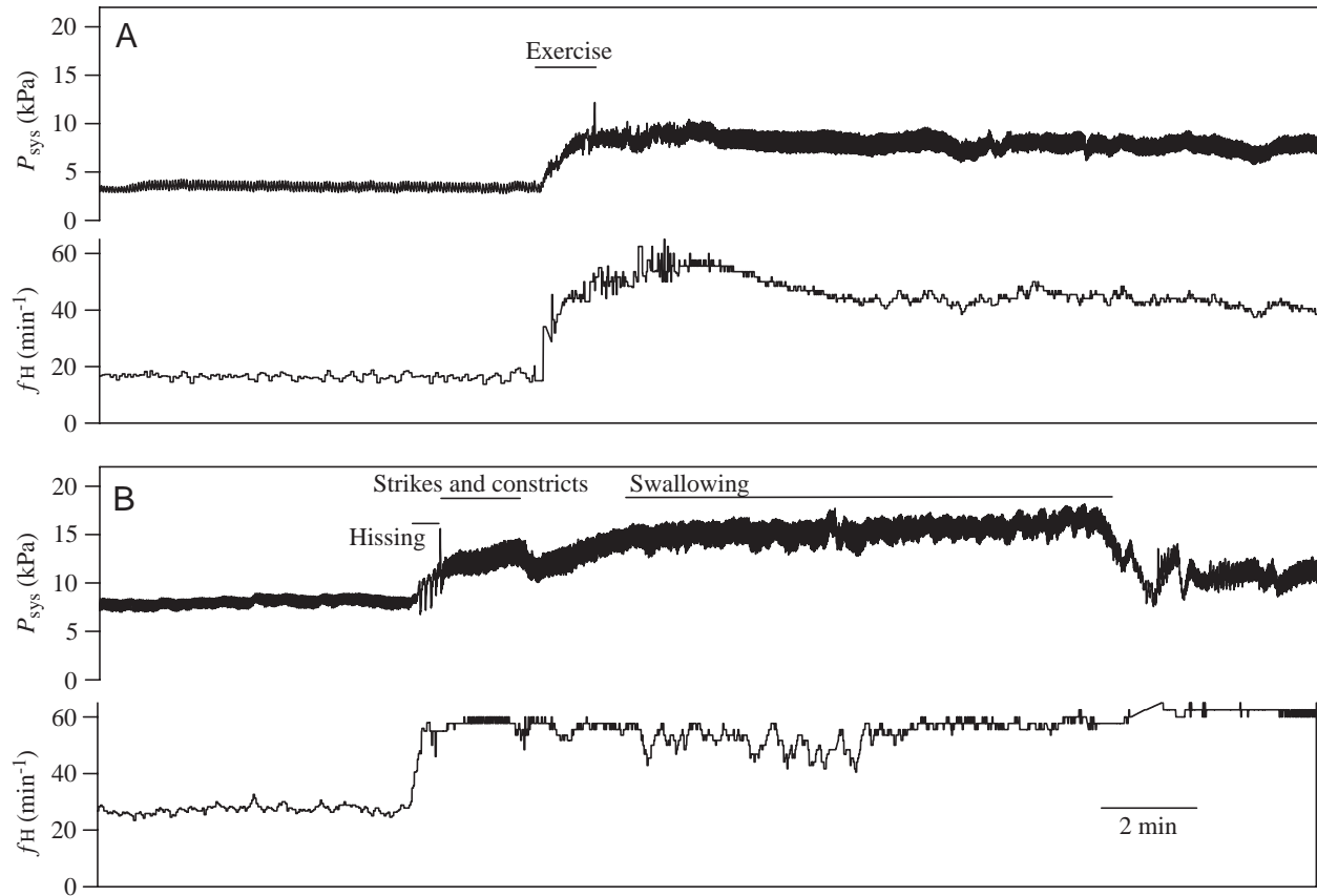
Fig. 1. Original recordings of heart rate ( f_H ) and systemic blood pressure ( P_{\text{sys}} ) in two different snakes used for the studies of enforced activity (A) and the effects of digestion (B).
