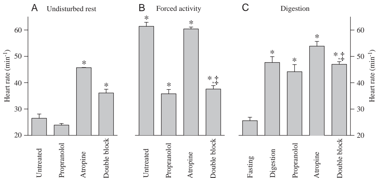
Fig. 3. Heart rate for Boa constrictor during resting and undisturbed conditions (A), during forced activity (B) and during digestion (C). The figure depicts the untreated control condition ( N=8 ) and the values obtained following autonomic blockade with the \beta -adrenergic antagonist propranolol ( 3 \text{ mg kg}^{-1} ) and the muscarinic cholinergic antagonist atropine ( 3 \text{ mg kg}^{-1} ; N=4 for both) and following double autonomic blockade ( N=8 ). The fasting heart rate is also shown for the snakes studied during digestion (C). Values are means + S.E.M. An asterisk indicates a significant difference from the value of untreated and resting animals; a double dagger indicates a significant difference from the value of double-blocked and resting animals.
