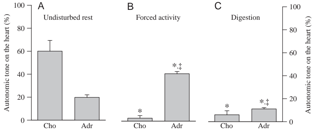
Fig. 4. The calculated autonomic tones on the heart for Boa constrictor during undisturbed rest (A), during forced activity (B) and during digestion (C). Values are means + S.E.M. An asterisk indicates a significant difference from the value of untreated and resting animals; a double dagger indicates a significant difference between forced activity and digestion. Cho, cholinergic; Adr, adrenergic.
