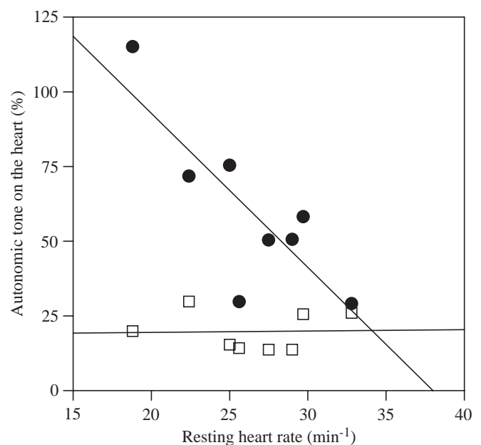
Fig. 5. Relationship between the heart rate of fasting, undisturbed and resting snakes and the cholinergic tone (filled circles) and the adrenergic tone (open squares) in Boa constrictor . The lines are linear regressions (cholinergic tone, r^2=0.663 , P=0.01 ; adrenergic tone, r^2<0.01 , P=0.94 ).
